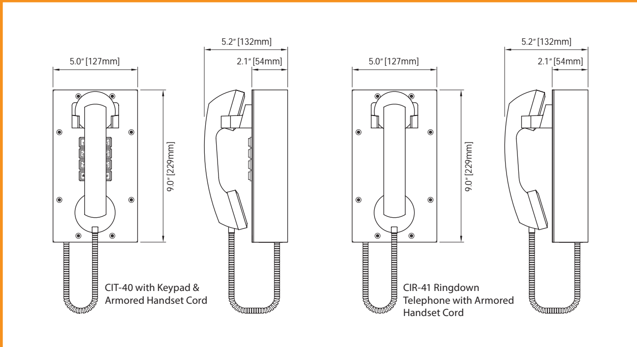
CIT-40 Correctional Institute Telephone • CIR-41 Correctional Institute Ringdown Telephone
