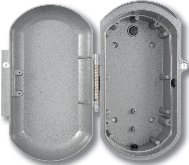
ACE-100 – Cast Aluminum Instrument Enclosure
