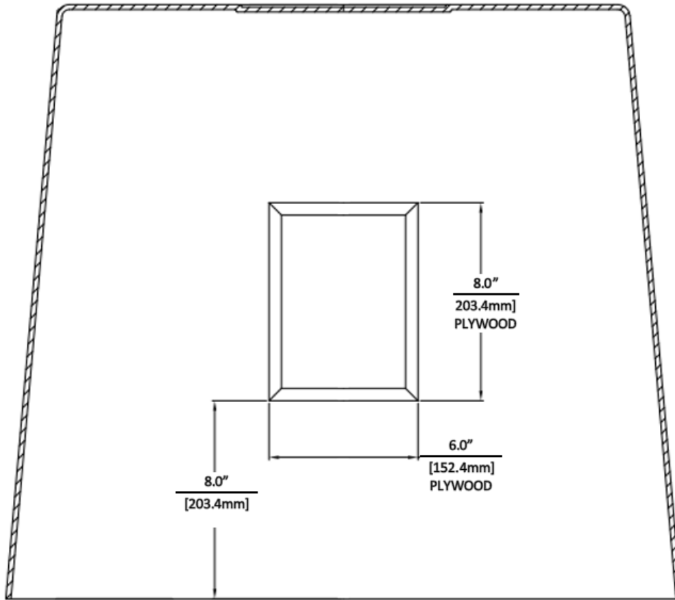
Figure 2 - Upper Mounting Location
