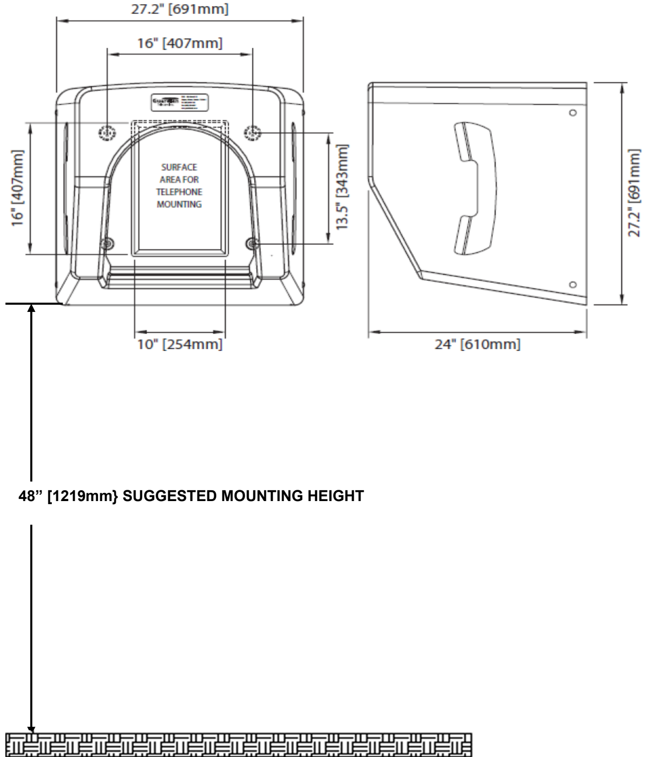
Figure 1 - Dimensions and Mounting
