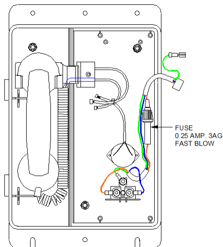
Figure 6 - Fuse Replacement
