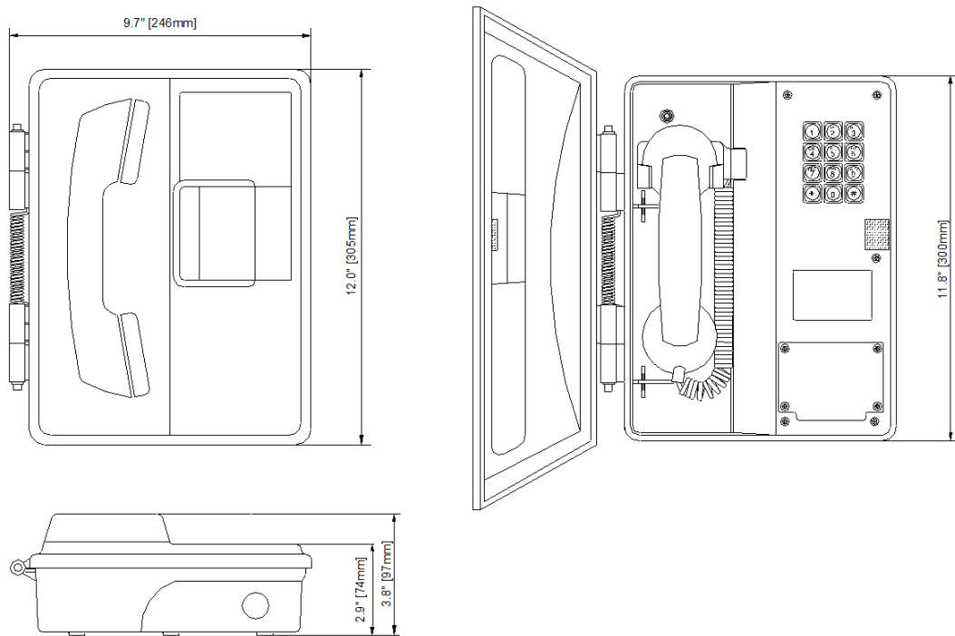
Figure 1 - Features - Typical - Standard Models
