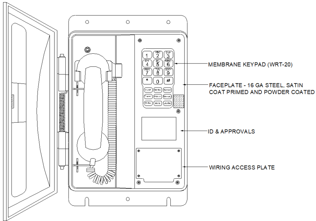
Figure 3 - Features WRT-20 with Optional Mounting Plate
