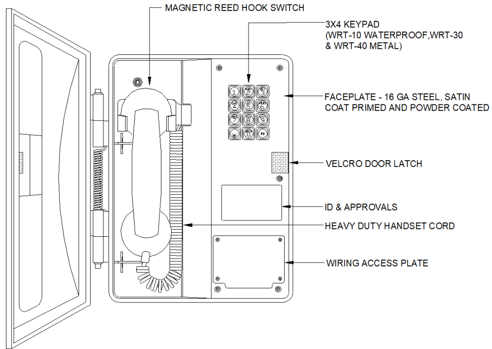
Figure 1 - Features - Typical - Standard Models
