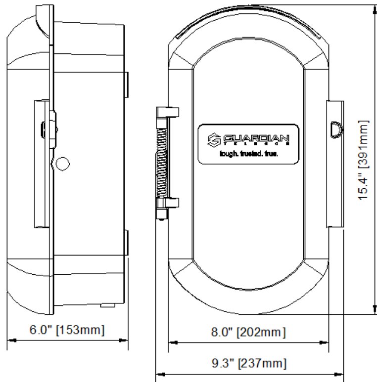
Figure 2 - Overall Dimensions
