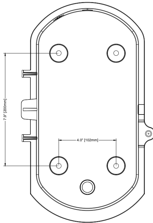
Figure 3 - Mounting
