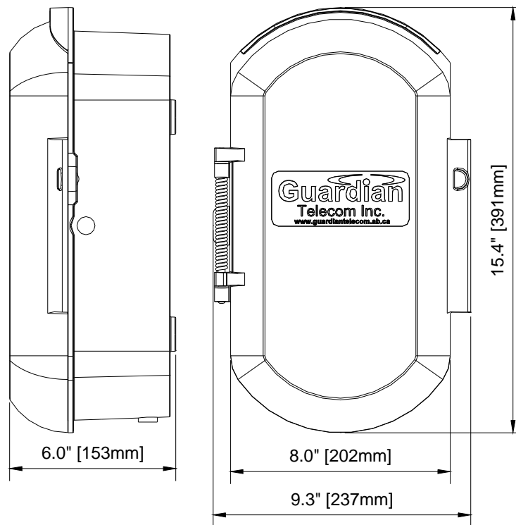
Figure 2 - Overall Dimensions
